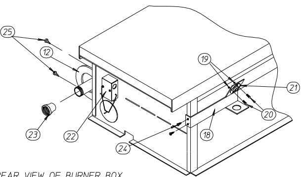
REAR VIEW OF BURNER BOX
